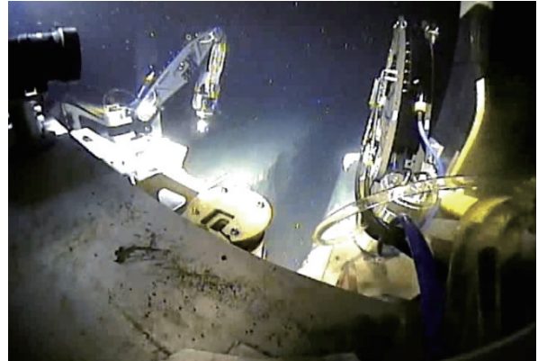
Sea Trial of URI-T: survey of cable burying results
